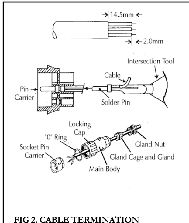
FIG 2. CABLE TERMINATION
